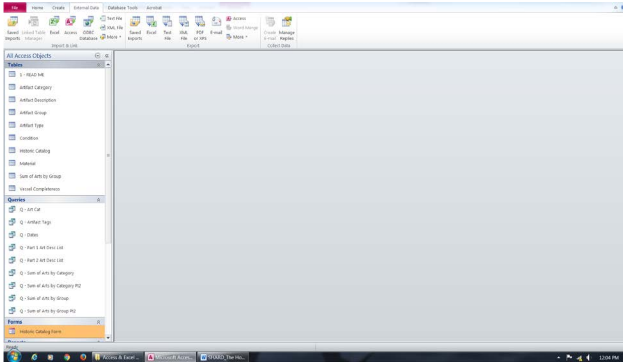
Figure 1. Opening Screen.
