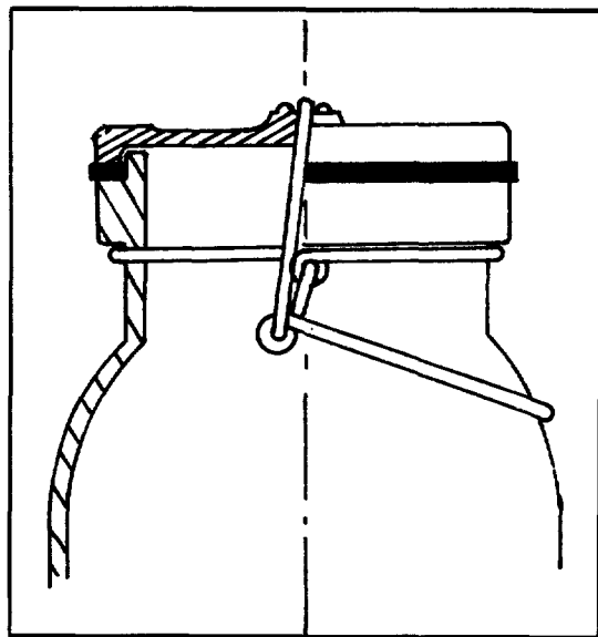
Figure 4d. Lightning type closure with iron bail and lever.
