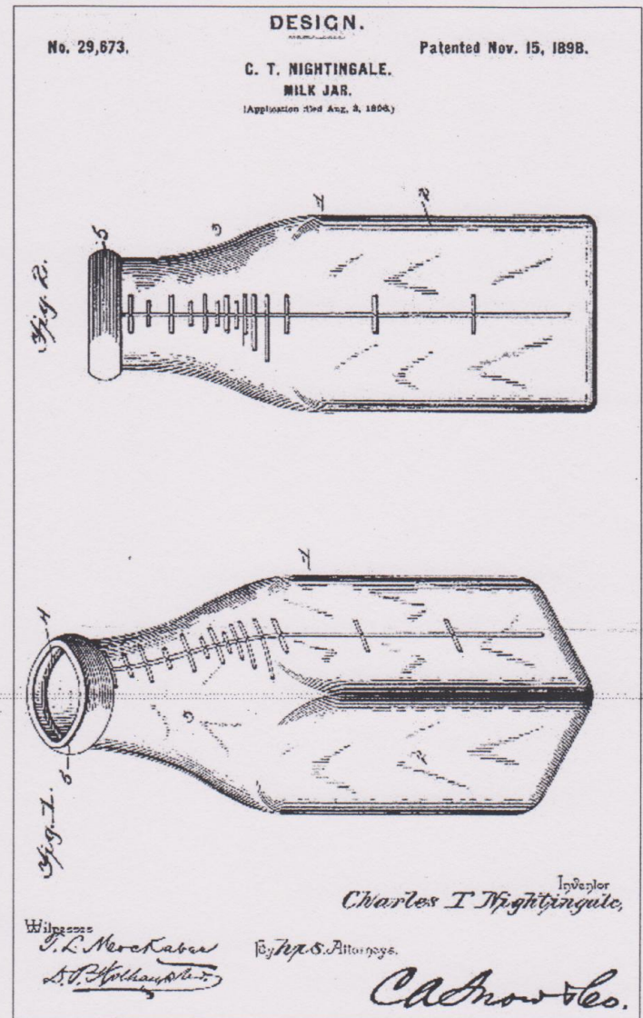
Fig. 2 - Nightingale's 1898 patent for a square milk bottle.
